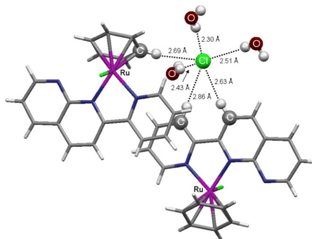
Fig. 5. Hydrogen-bonded network observed in [1]Cl · 3H 2 O with H–Cl distances.
