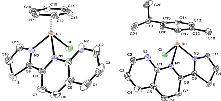
Fig. 4. ORTEP diagram of cations 2 (left) and 5 (right) at 50% probability level with anion and H atoms being omitted for clarity.
